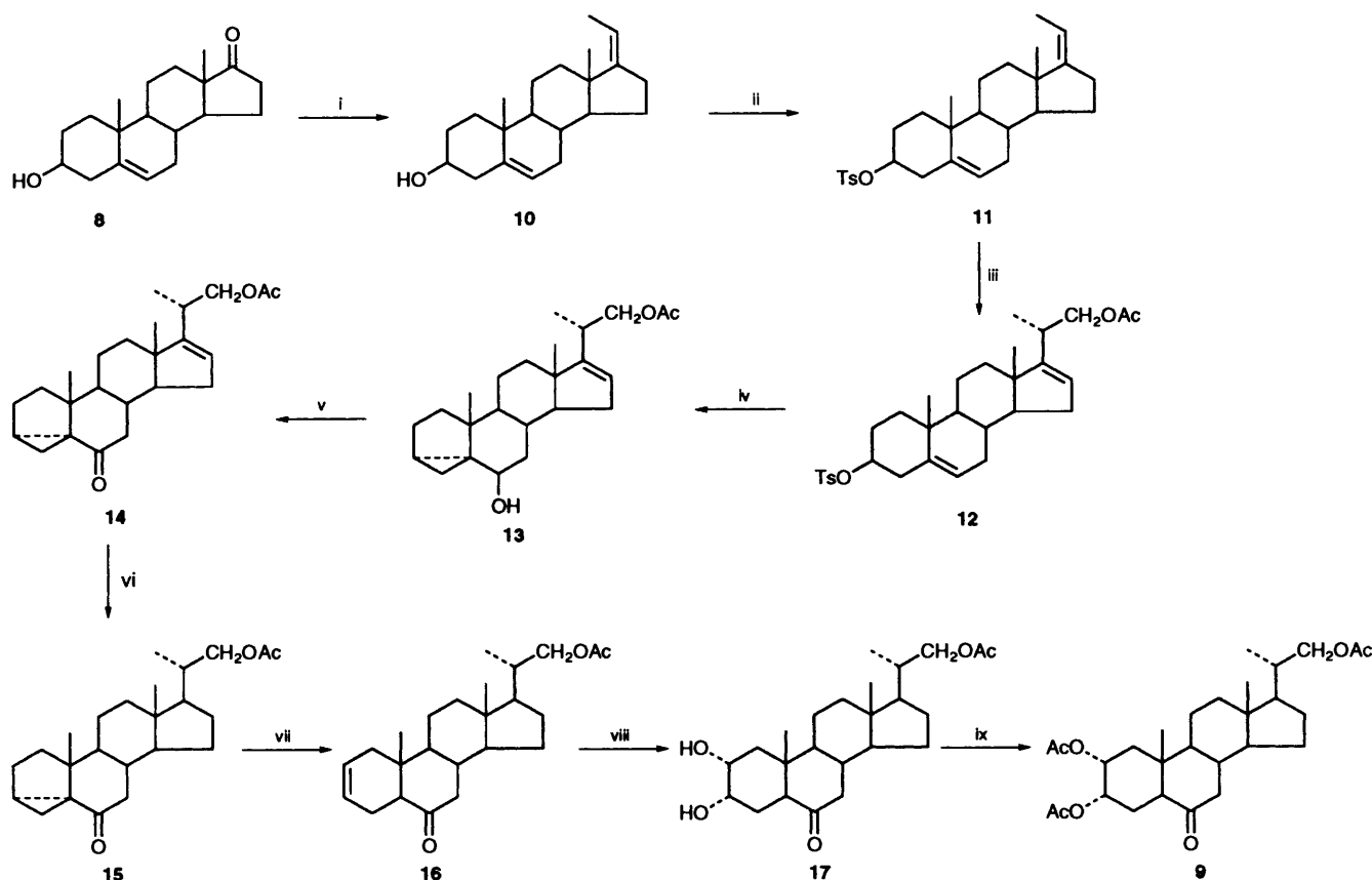
Scheme 1 Reagents and conditions: i, \text{Ph}_3\text{P}^+\text{Et I}^- , \text{KOBU}^+ , \text{Bu}^+\text{OH} , reflux, 6.5 h (89%); ii, 4-MeC 6 H 4 SO 2 Cl, py, 25 °C, 48 h (90%); iii, resin, (CH 2 O) n , Ac 2 O, CH 2 Cl 2 , 25 °C, 20 h (96%); iv, KOAc, acetone-water, reflux, 3 h (88%); v, CrO 3 , acetone, 10 °C, 0.5 h (86%); vi, Pd/C H 2 , EtOH, 25 °C, 6 h (98%); vii, PPTS, LiBr, DMF, reflux, 4 h (80%); viii, OsO 4 , NMO, Bu + OH, acetone, 25 °C, 1.5 h (98%); ix, py, Ac 2 O, 60–65 °C, 8 h (99%).
